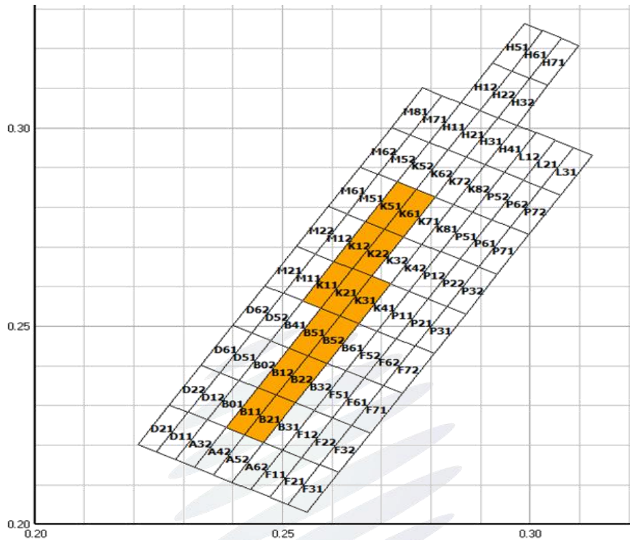
Fig. 1-6 The C.I.E Chromaticity Diagram CIE色度图
