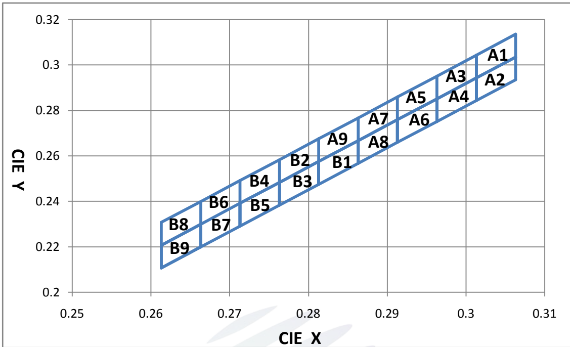
Fig. 1-6 The C.I.E Chromaticity Diagram CIE色度图
