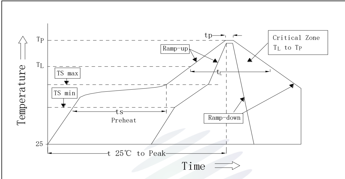
Fig.3-1 SMT Reflow Soldering Instructions SMT 回流焊说明
