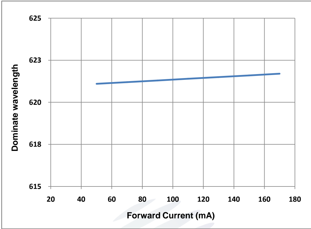
Fig. 1-13 Forward current vs. Dominate wavelength正向电流与主波长特性曲线 (Ts=25°C)
