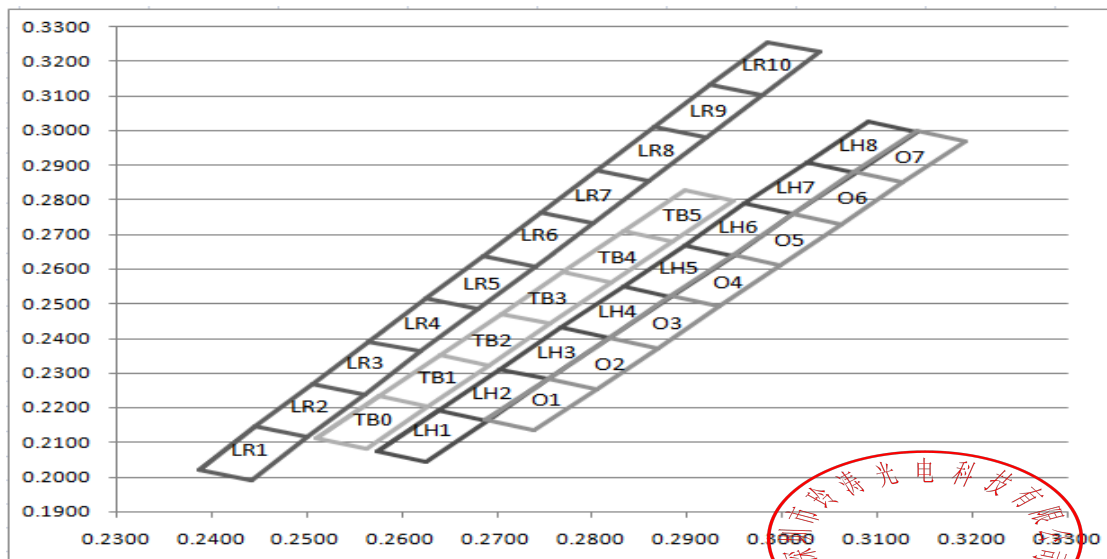
Fig. 1-9 The C.I.E. 1931 Chromaticity Diagram: ( LR&TB&LH&O 色系 )
