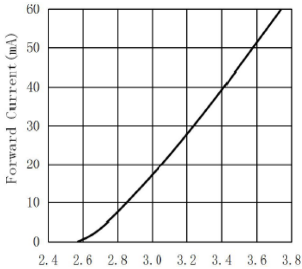
Fig. 1-13 Forward Voltage Vs Forward Current 伏安特性曲线
