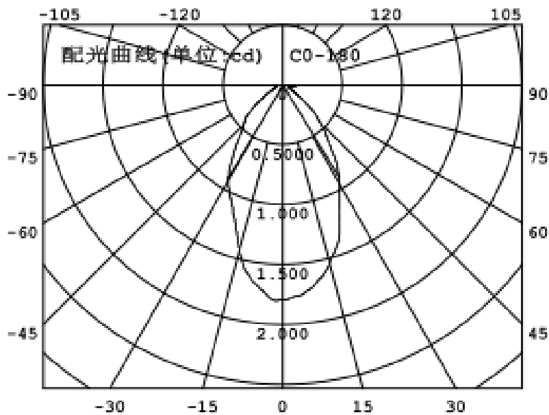
Fig.1-13 Diagram characteristics of radiation 辐射特性曲线
